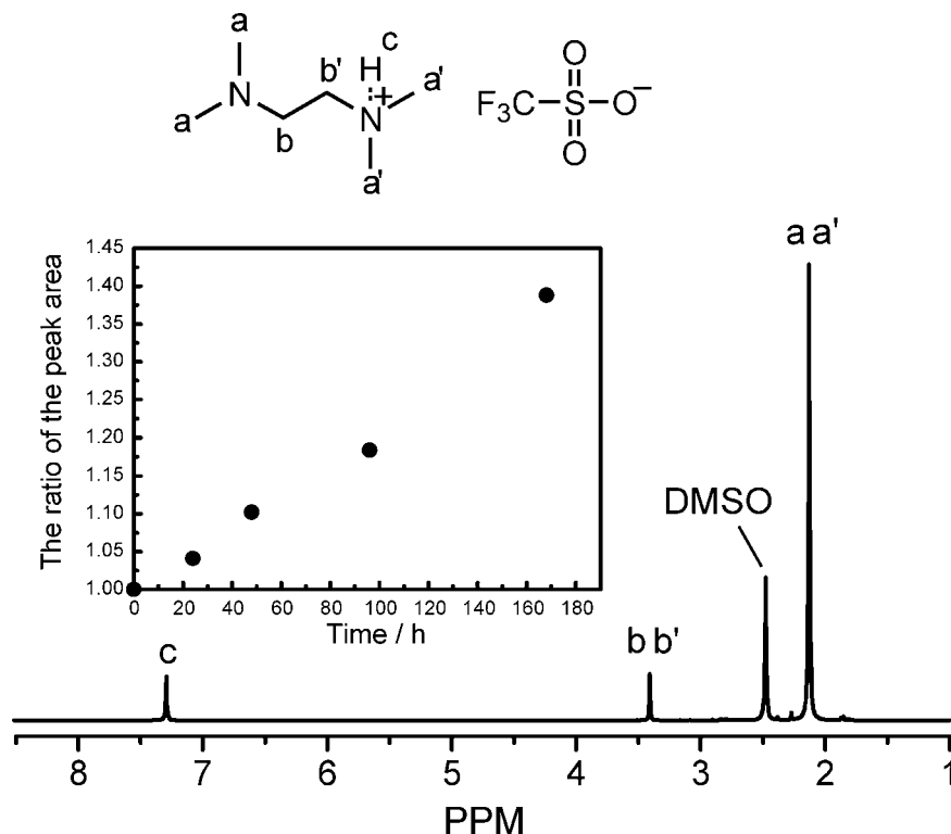
Figure 5. ^1\text{H} NMR spectrum of [temeda][TfO]. The inset shows a change in the ratio of 1/12 (corresponding to the single proton) of the integrated methyl protons ( a + a' ) to the integrated ammonium proton ( c ) when [temeda][TfO] is evacuated at 120^\circ\text{C} .
