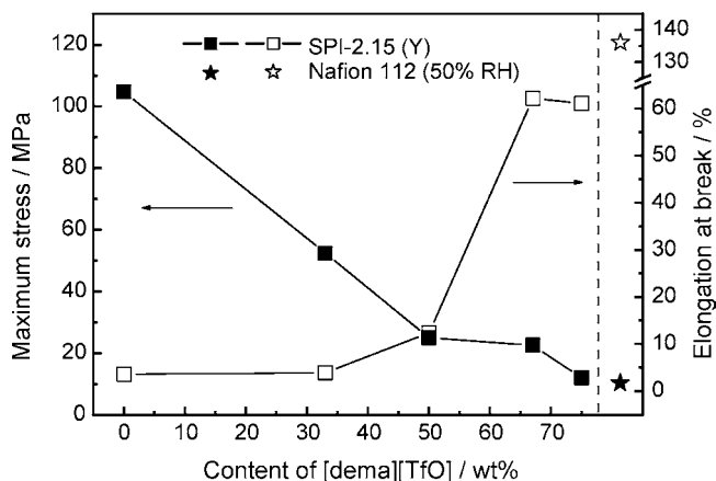
Figure 6. Tensile strength and elongation at break of SPI-2.15 composite membranes as a function of [dema][TfO] content at room temperature. The data for Nafion 112 at room temperature are cited from ref 32.
