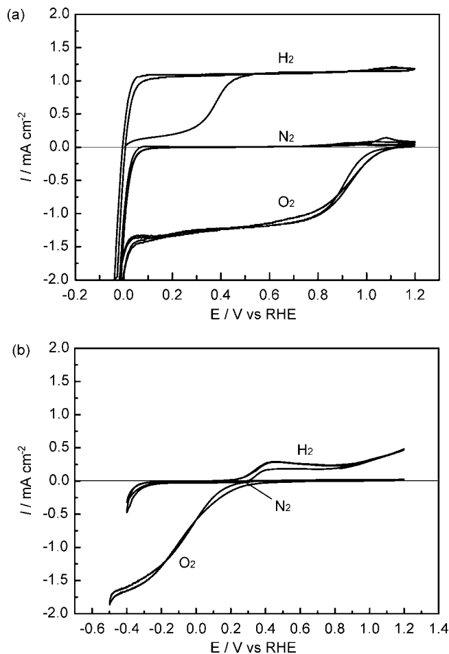
Figure 3. Cyclic voltammograms of (a) [dema][TfO] and (b) [dema][NTf 2 ] using a Pt wire working electrode under H 2 , O 2 , or N 2 gas bubbling conditions. Scan rate is 10 mV s -1 , and gas feed is 2 mL min -1 . The voltammogram for [dema][NTf 2 ] is cited from ref 27.
